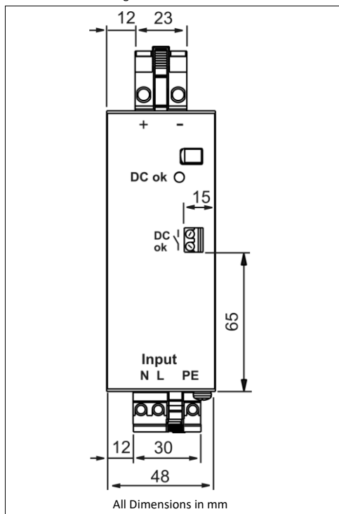
Fig. 22-1 Front view
