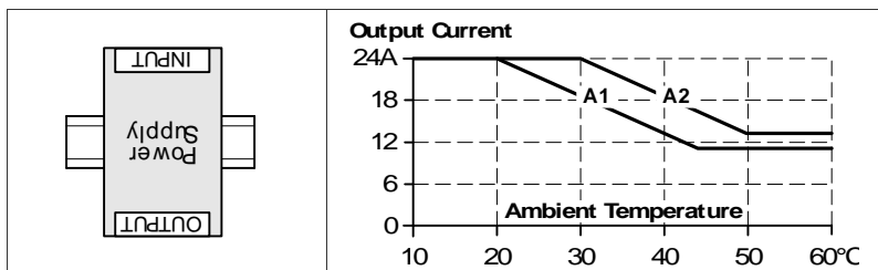
Fig. 24-10 Mounting Orientation B (Upside down)
