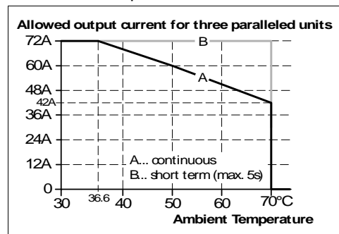
Fig. 24-6 Output current vs. ambient temp. for three paralleled units
