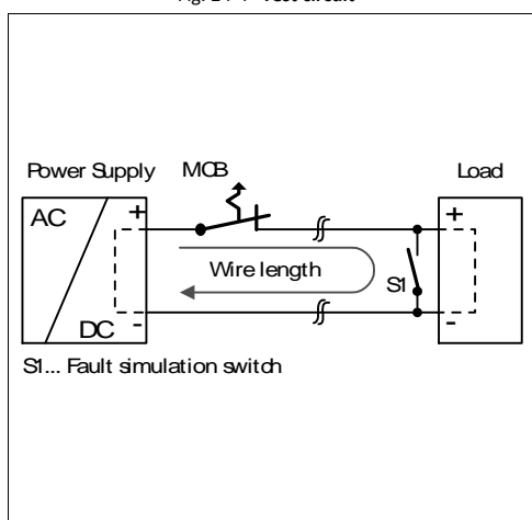
Fig. 24-4 Test circuit
