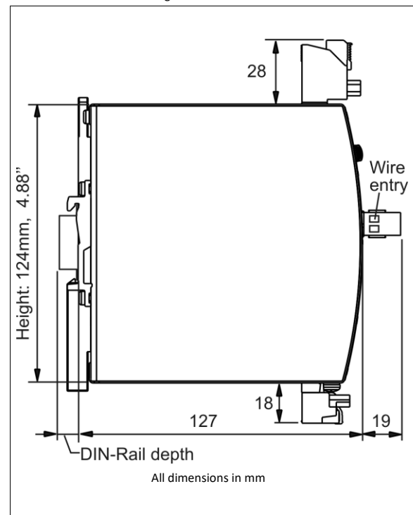
Fig. 22-2 Side view
