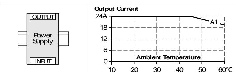
Fig. 24-9 Mounting Orientation A (Standard orientation)
