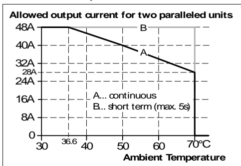
Fig. 24-5 Output current vs. ambient temp. for two paralleled units
