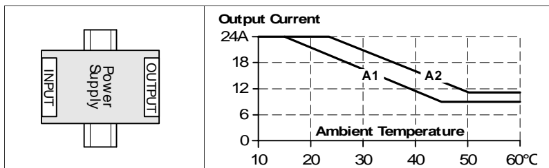
Fig. 24-12 Mounting Orientation D (Horizontal cw)
