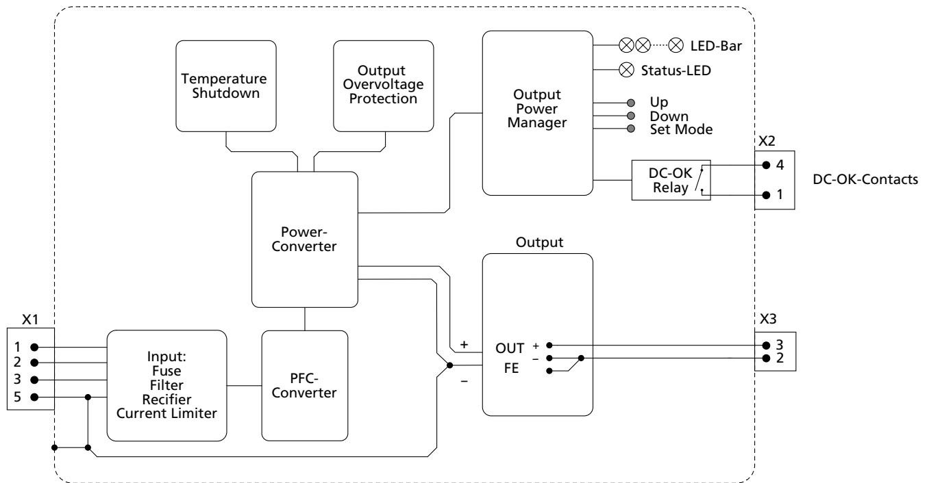
Fig. 12-1: Functional Diagram FPT500.241-010-108
