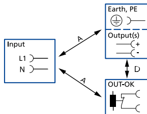
Fig. 18-1: Dielectric strength
