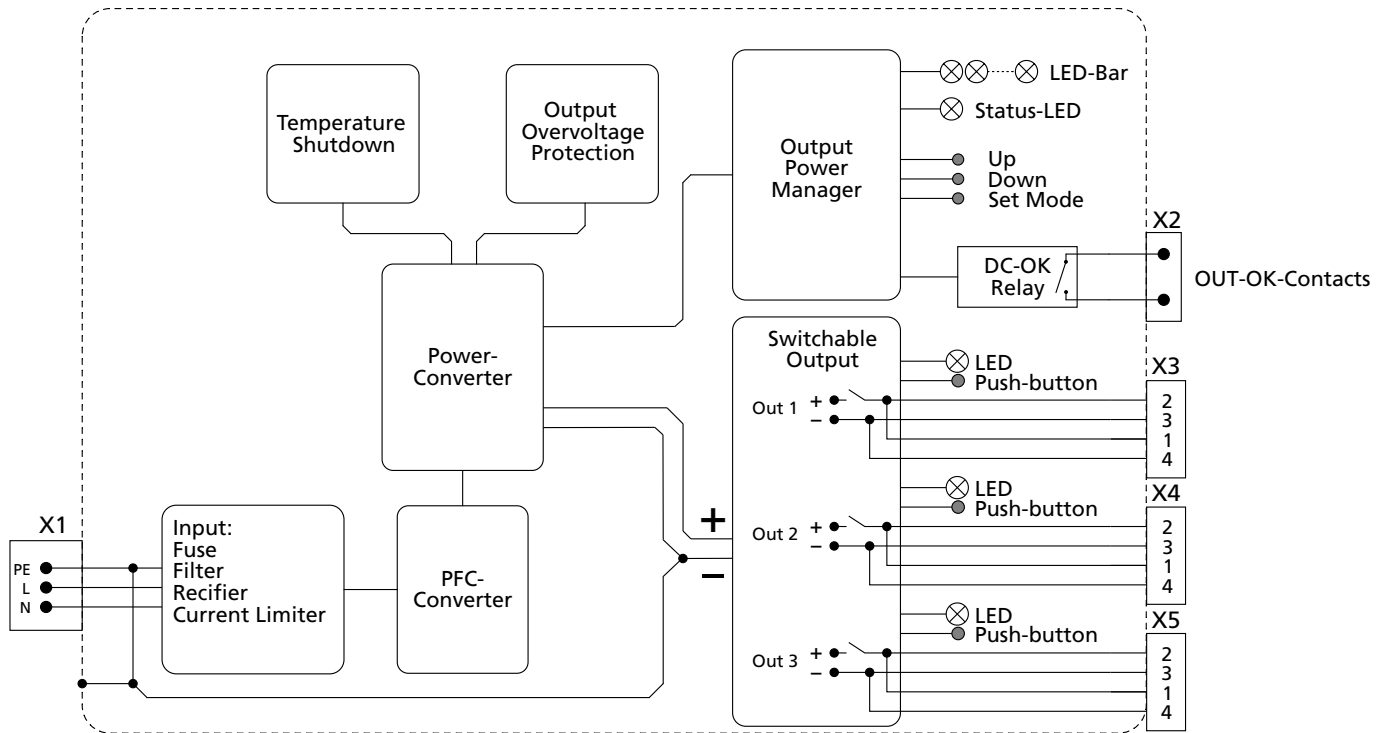
Fig. 12-1: Functional Diagram FPS300.245-049-102
