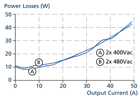
Fig. 29-4: Power Losses vs. output current at 24 V
