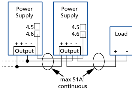
Fig. 17-1: Daisy chaining of outputs
