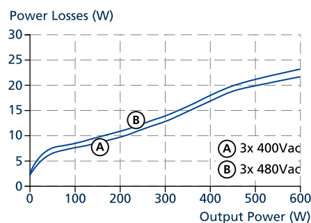
Fig. 9-2: Losses vs. output power at 48 V, typ.
