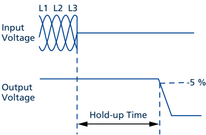
Fig. 7-2: Shut-down behavior, definitions
