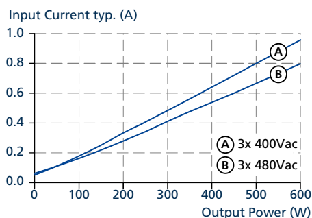
Fig. 3-3: Input current vs. output power at 48 V output voltage
