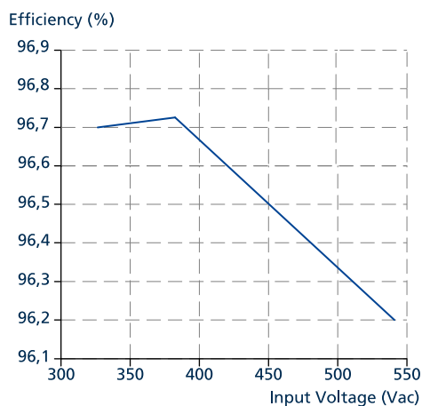
Fig. 9-3: Efficiency vs. input voltage at 48 V, 500 W, typ.
