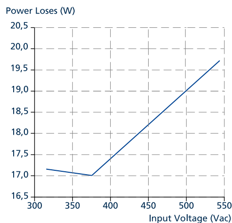
Fig. 9-4: Losses vs. input voltage at 48 V, 500 W, typ.
