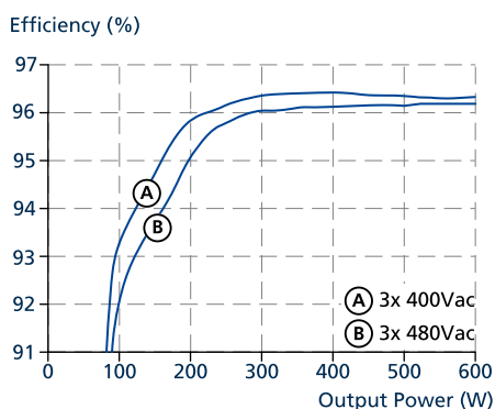
Fig. 9-1: Efficiency vs. output power at 48 V, typ.
