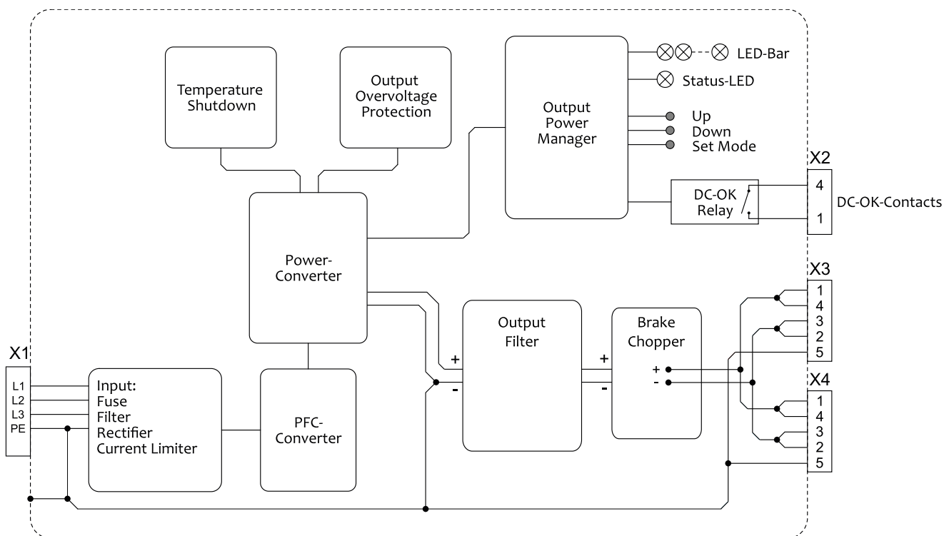
Fig. 12-1: Functional Diagram FPT500.481-034-103
