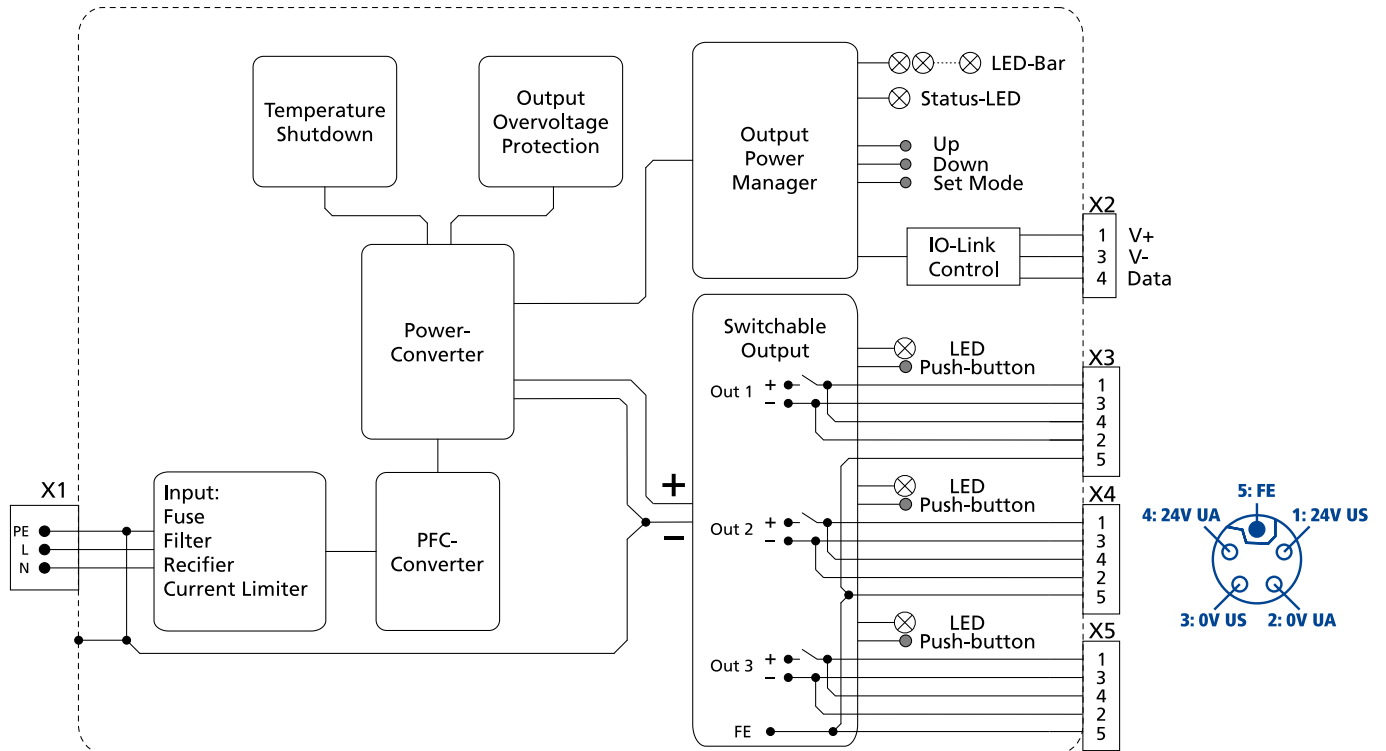
Fig. 12-1: Functional Diagram FPH500.245-024-103
