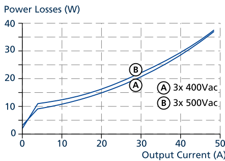
Fig. 13-2: Losses vs. output current at 24 V, typ.
