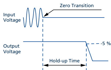
Fig. 7-2: Shut-down behaviour
