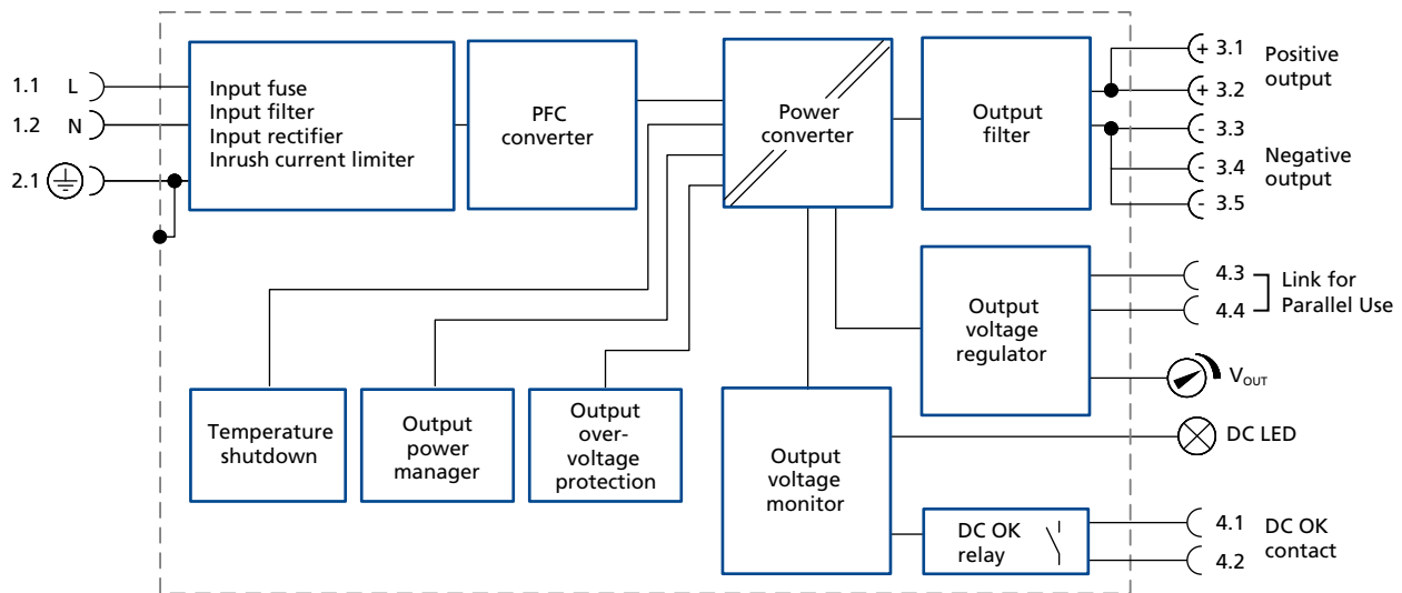
Fig. 12-1: Functional Diagram SP960.481-S
