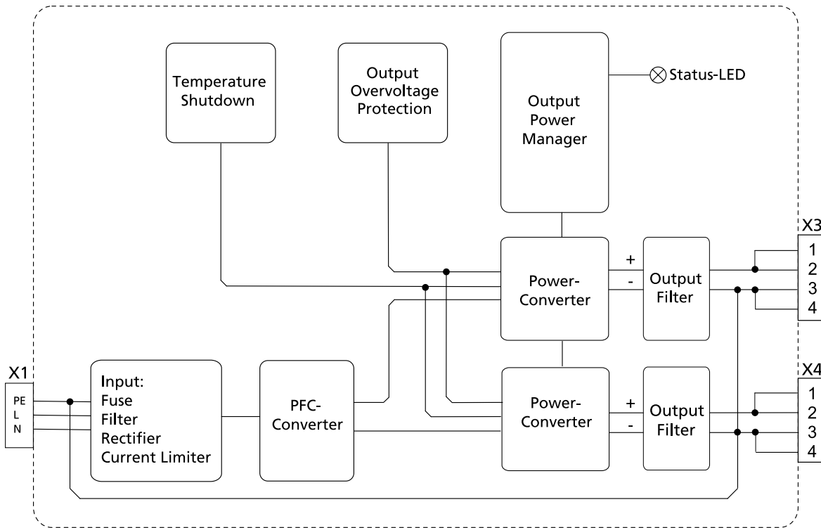
Fig. 12-1: Functional Diagram FPS202.241-011
