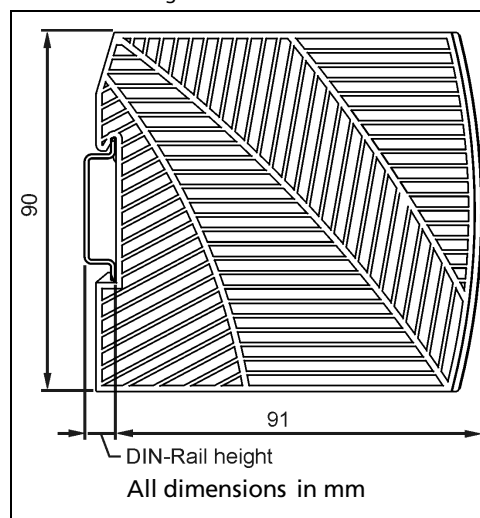
Fig. 20-2 Side view
