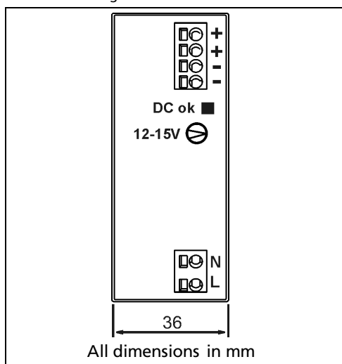
Fig. 20-1 Front view
