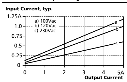
Fig. 3-3 Input current vs. output load at 12V output voltage
