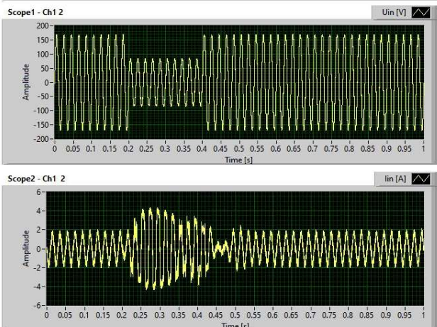
25°C Norm 120V 50Hz 0.200s 50% L1-N 0°
