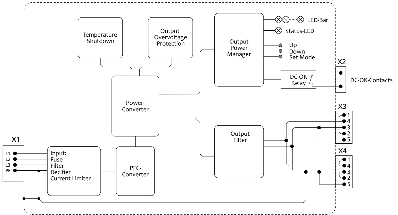
Fig. 12-1: Functional Diagram FPT500.481-034-103
