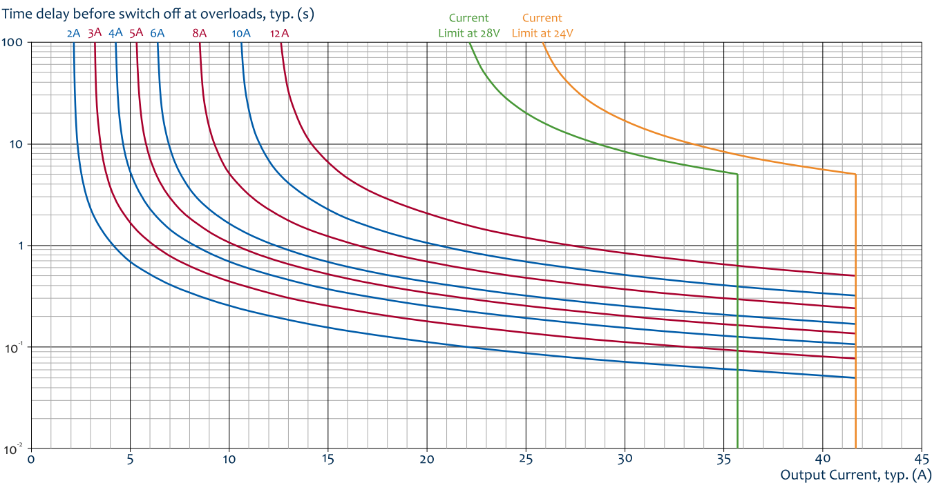
Fig. 6-2: Tripping curve diagram
