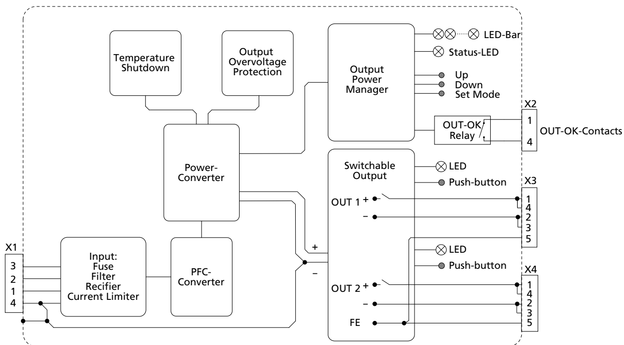
Fig. 12-1: Functional Diagram FPT500.245-070-162
