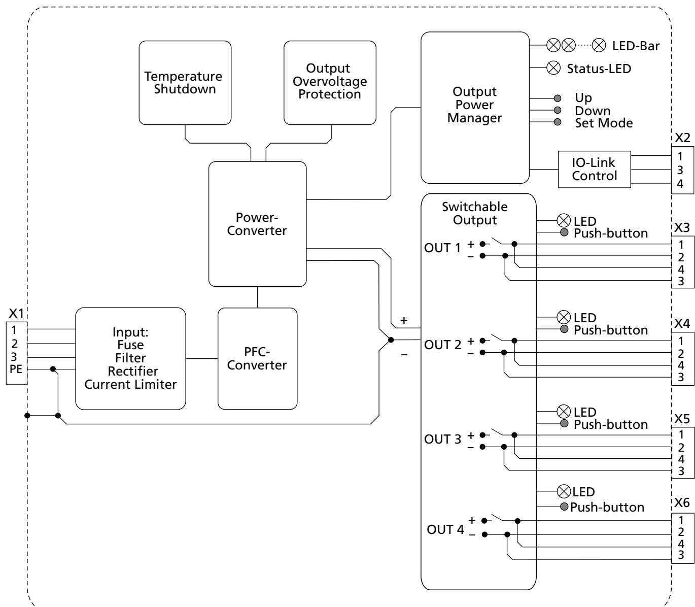
Fig. 12-1: Functional Diagram FPT500.245-044-109
