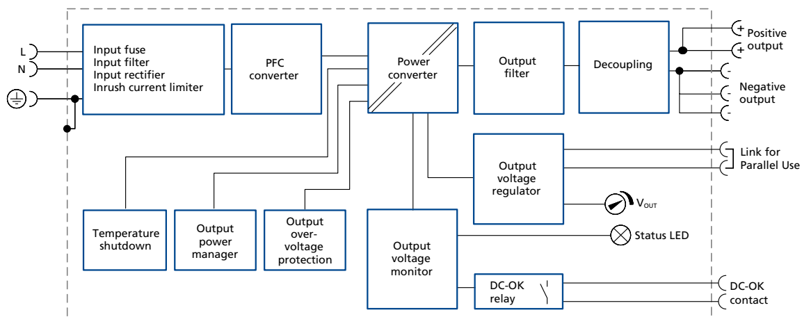
Fig. 12-1: Functional Diagram SP960.241-SR
