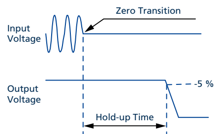
Fig. 7-2: Shut-down behaviour
