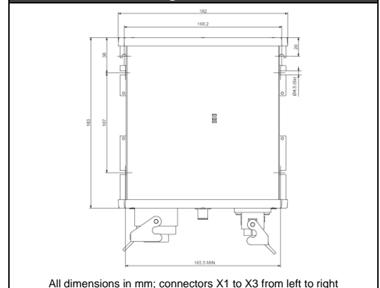
All dimensions in mm; connectors X1 to X3 from left to right
