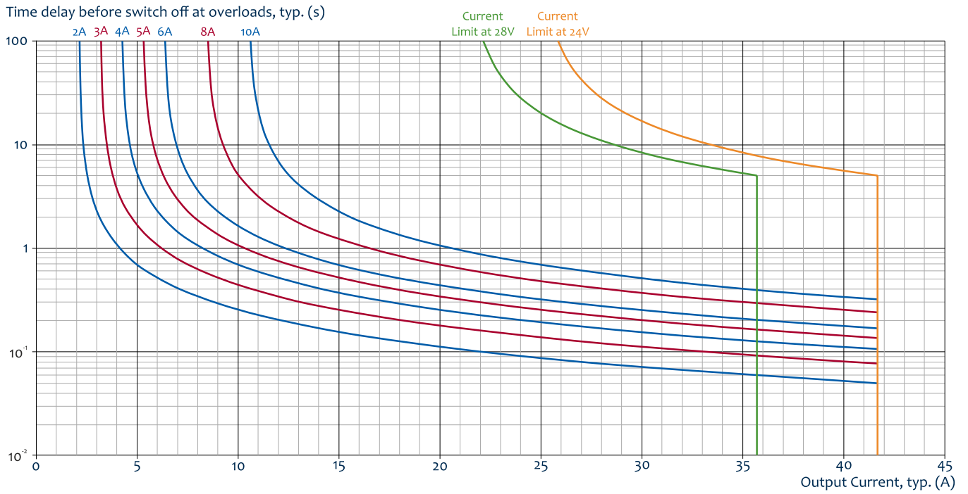
Fig. 6-2: Tripping curve diagram
