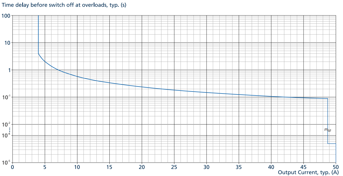
Fig. 6-3: Tripping curve diagram for NEC Class 2
