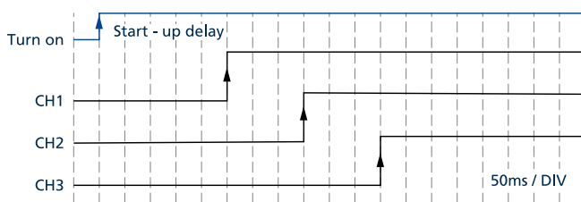
Fig. 6-1: Sequential start of the outputs
