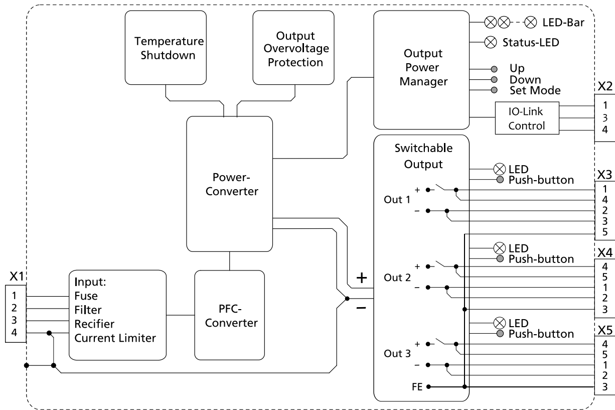
Fig. 12-1: Functional Diagram FPT500.247-064-102
