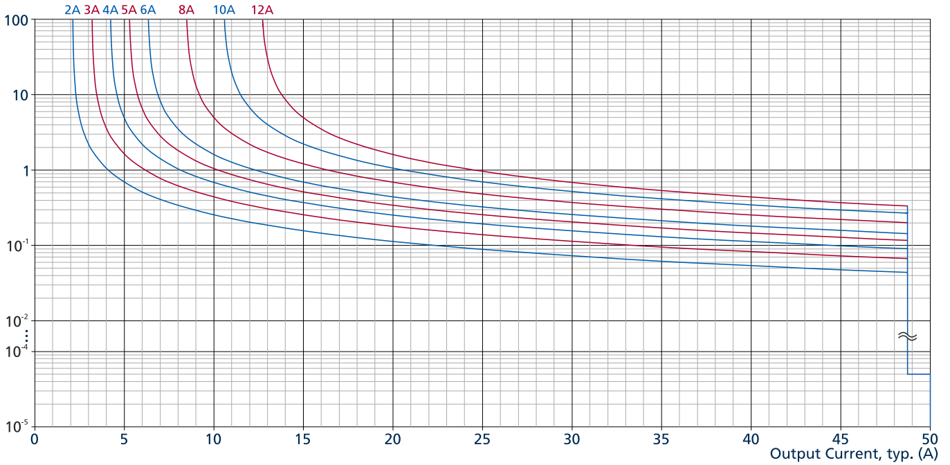
Fig. 6-2: Tripping curve diagram
