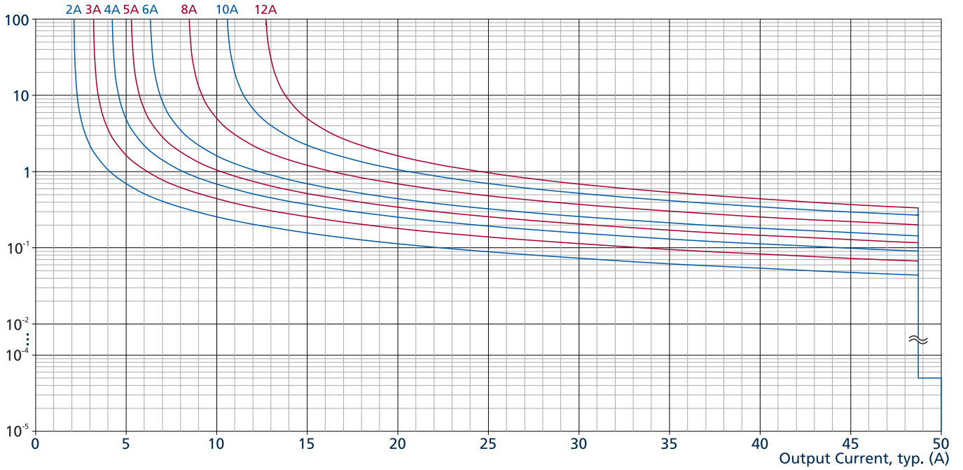
Fig. 6-3: Tripping curve diagram
