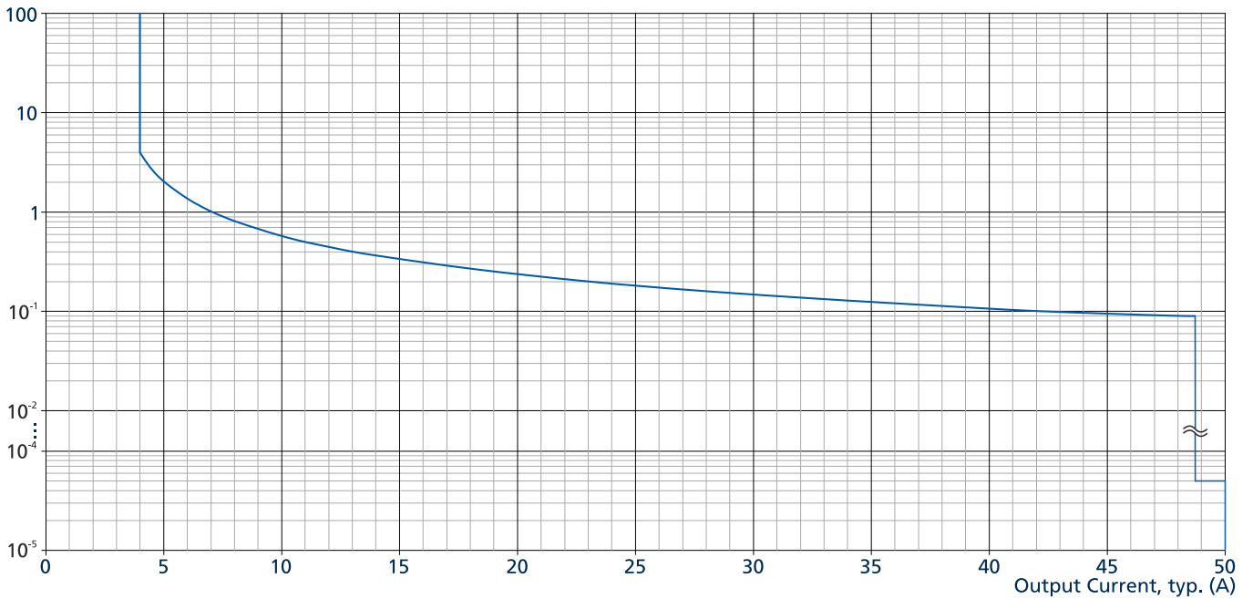
Fig. 6-4: Tripping curve diagram for NEC Class 2
