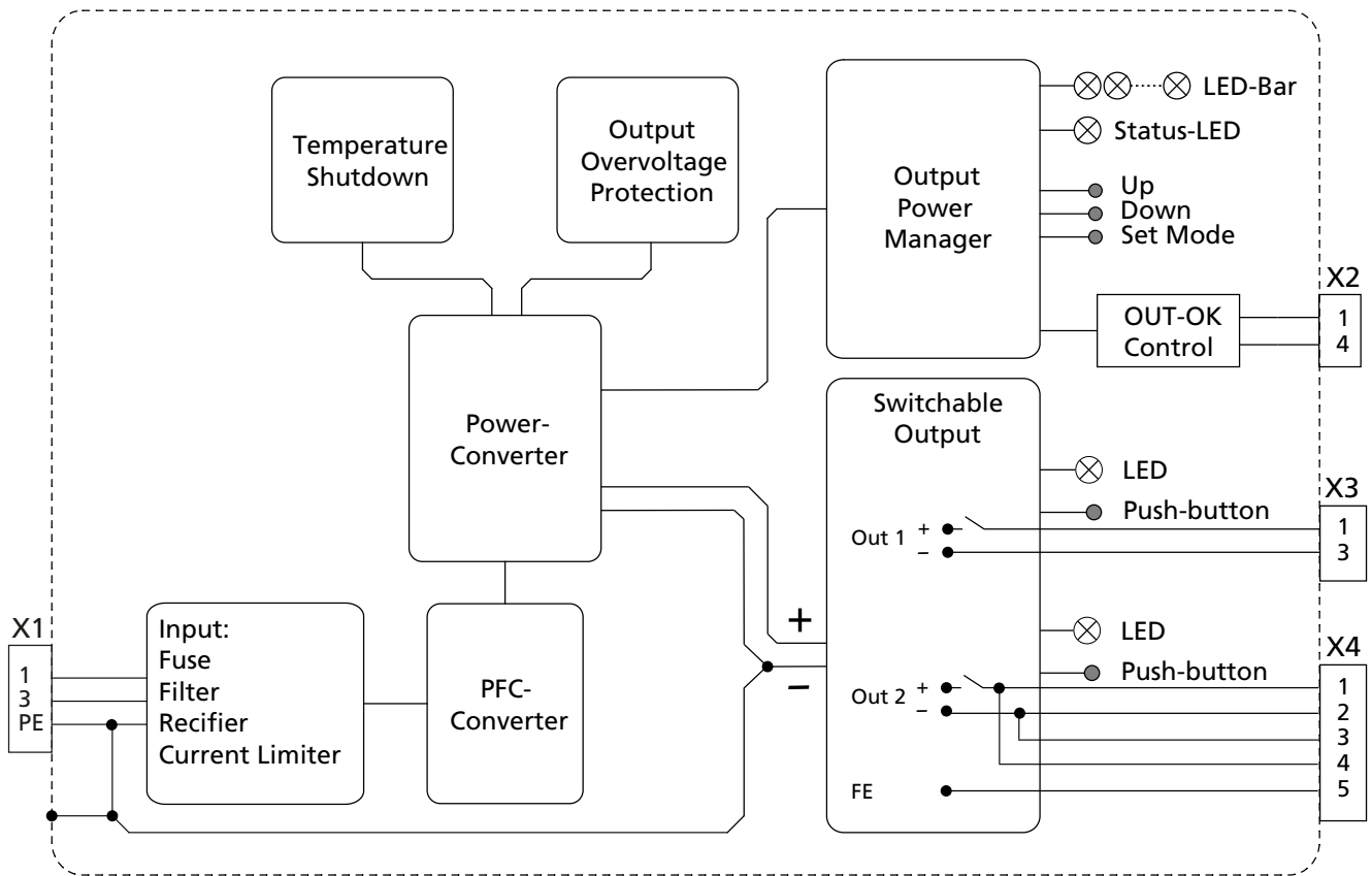
Fig. 12-1: Functional Diagram FPS300.247-060-101
