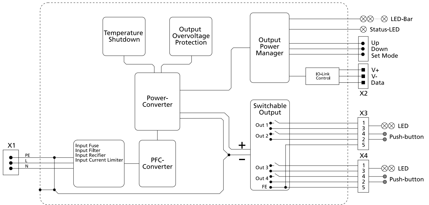
Fig. 12-1: Functional Diagram FPS300.245-034-105
