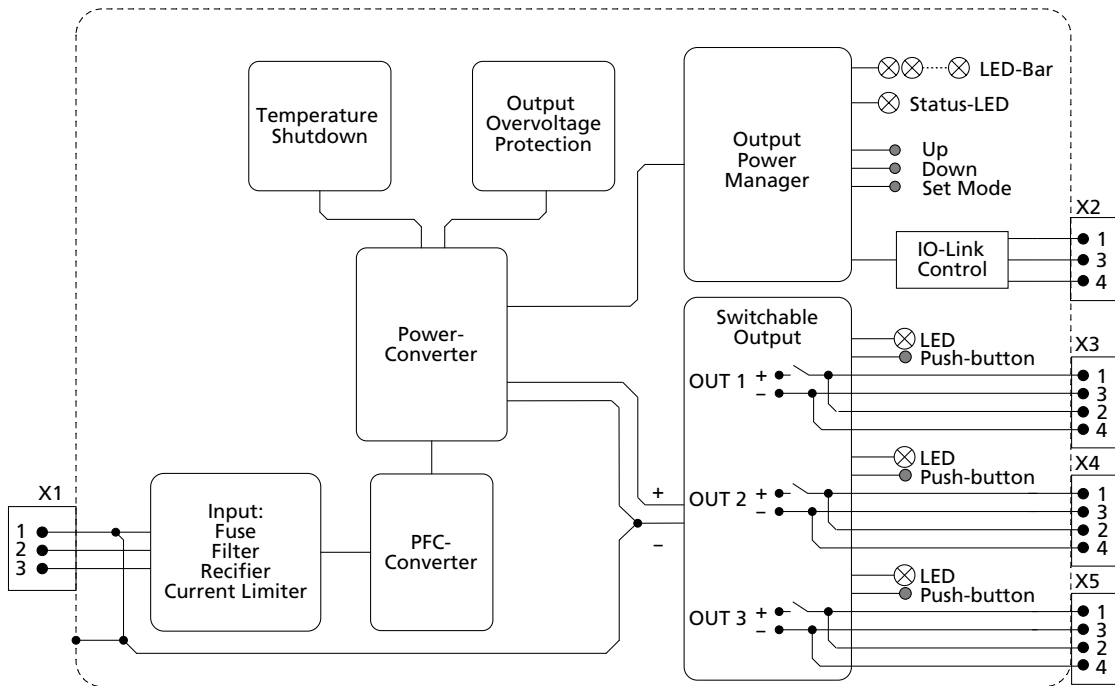
Fig. 12-1: Functional Diagram FPS300.246-049-102
