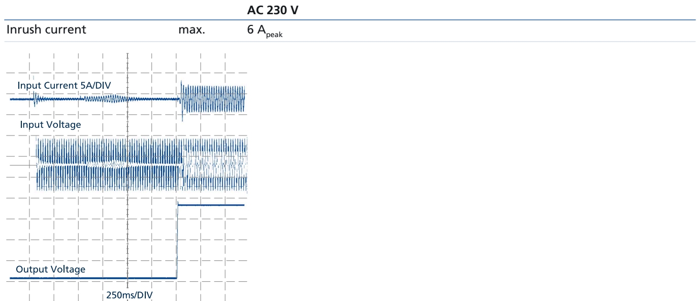
Fig. 5-1: Typical turn-on behavior at nominal load and +25 °C ambient temperature
