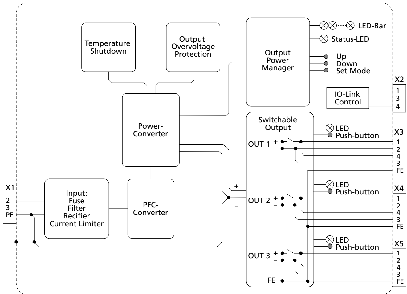
Fig. 12-1: Functional Diagram FPH500.245-024-103
