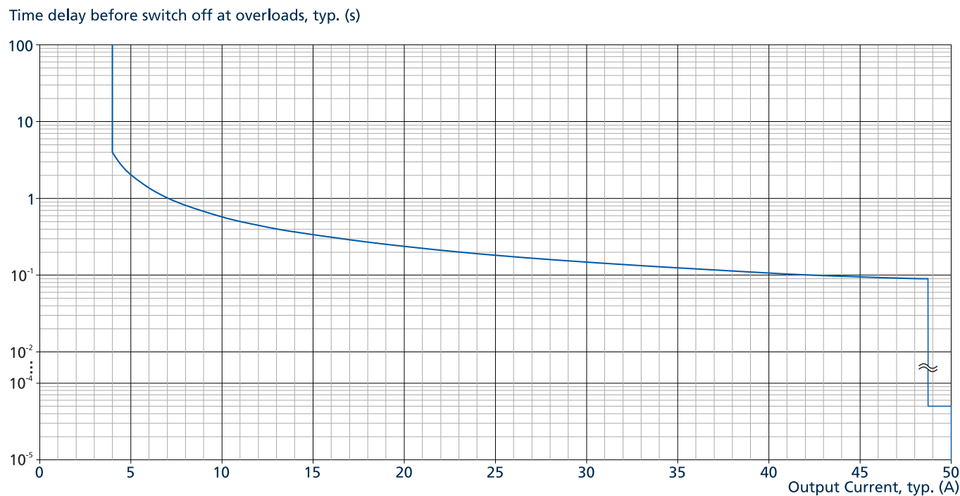
Fig. 6-4: Tripping curve diagram for NEC Class 2
