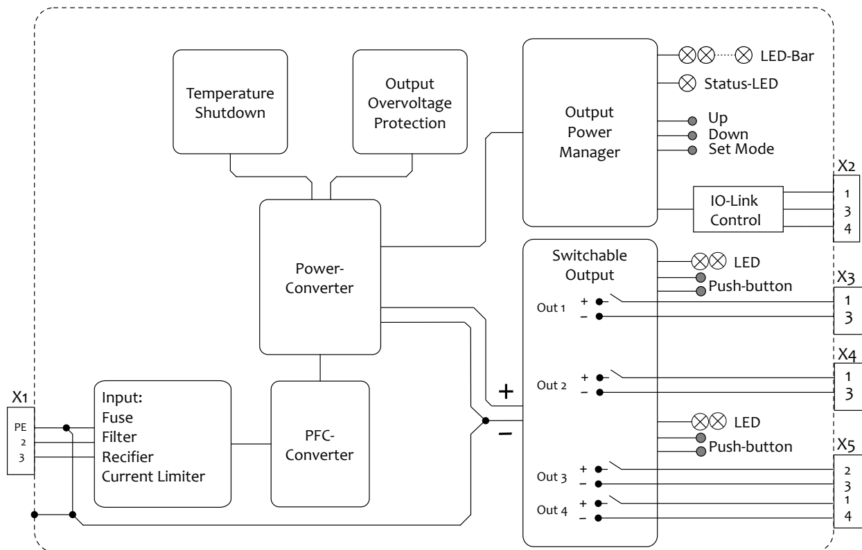
Fig. 12-1: Functional Diagram FPS300.247-071-151
