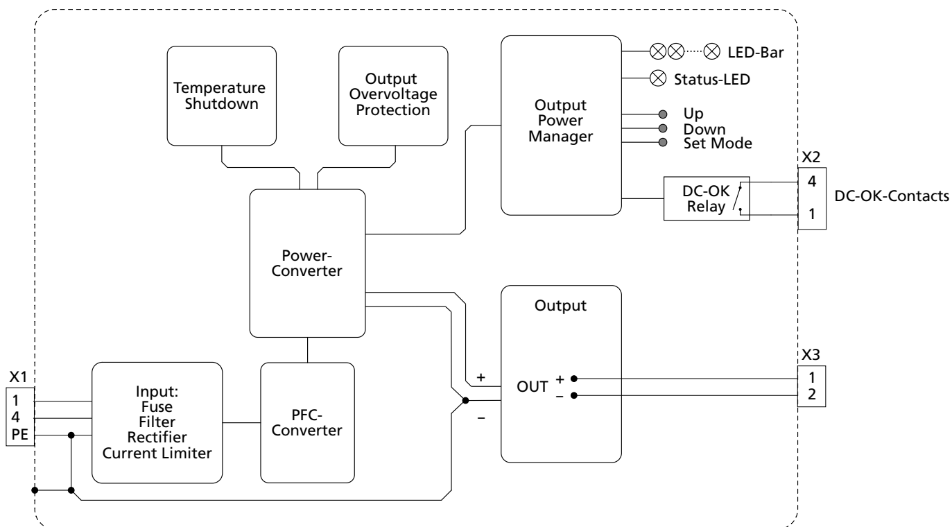
Fig. 12-1: Functional Diagram FPS300.241-010-104
