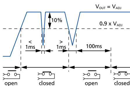
Fig. 8-1: Output-OK relay contact behavior
