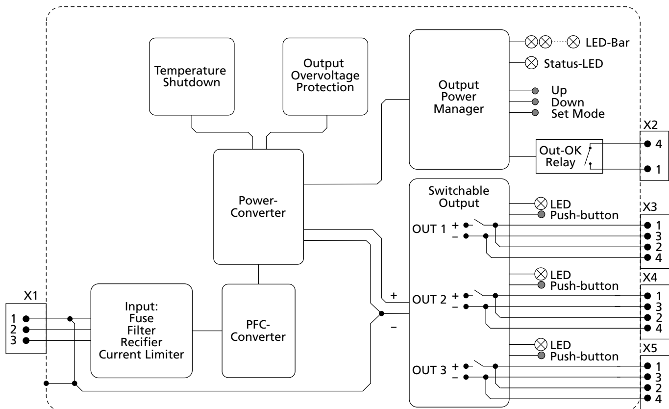
Fig. 12-1: Functional Diagram FPS300.246-049-106
